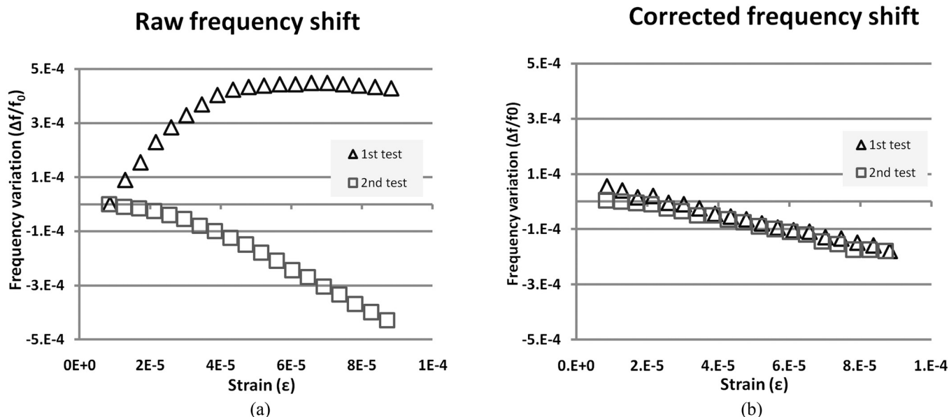
FIG. 2. Bone sample, first mode. (a) Frequency shift computed with Eq. (2) obtained during two different NRUS experiments. (b) Corrected frequency shift computed with Eq. (2) where f_0 is replaced by f_{0,n} . Temperature effects, if uncorrected, may result in frequency shifts (a) that overpass intrinsic nonlinear frequency shifts (b).
